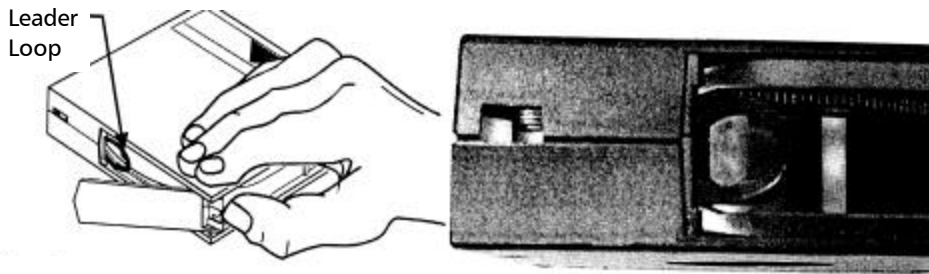
Figure D-3 Opening the Door on a DLTtape Cartridge Showing Tape Leader Loop in its Correct Position
